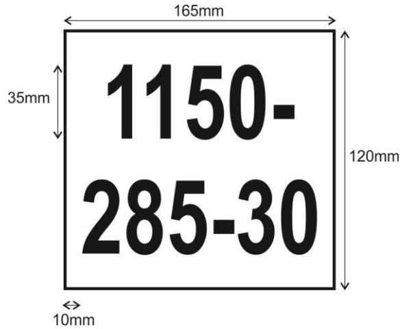
Diagram 2a) – Vehicle Markings Placement
